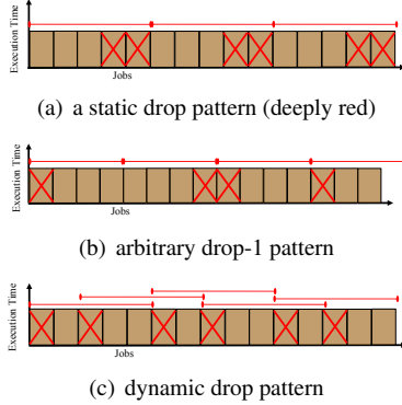
Figure 2. Firm real-time process with (3, 5) constraints using different drop patterns
