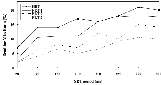
Figure 4. Firm real-time dropping pattern impact on soft real-time performance
